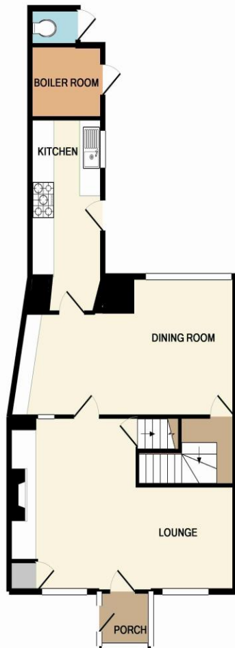
GROUND FLOOR APPROX. FLOOR AREA 628 SQ.FT. (58.4 SQ.M.)
