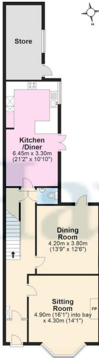
Ground Floor Approx. 83.8 sq. metres (901.7 sq. feet)
