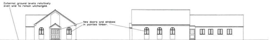
SOUTH ELEVATION 1:100.
