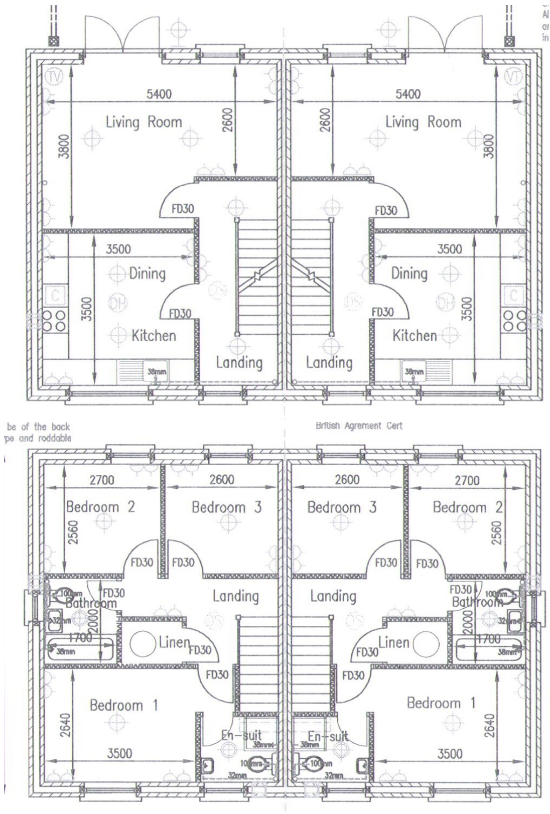
Floor layout plan for illustration purposes only. Whilst every attempt has been made to ensure the accuracy, all measurements are approximate and no responsibility is taken for errors and omissions.
