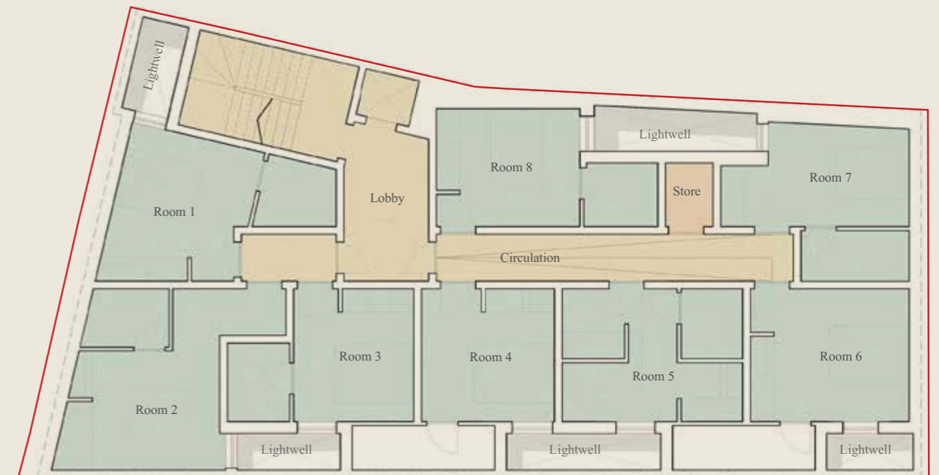
Basement
