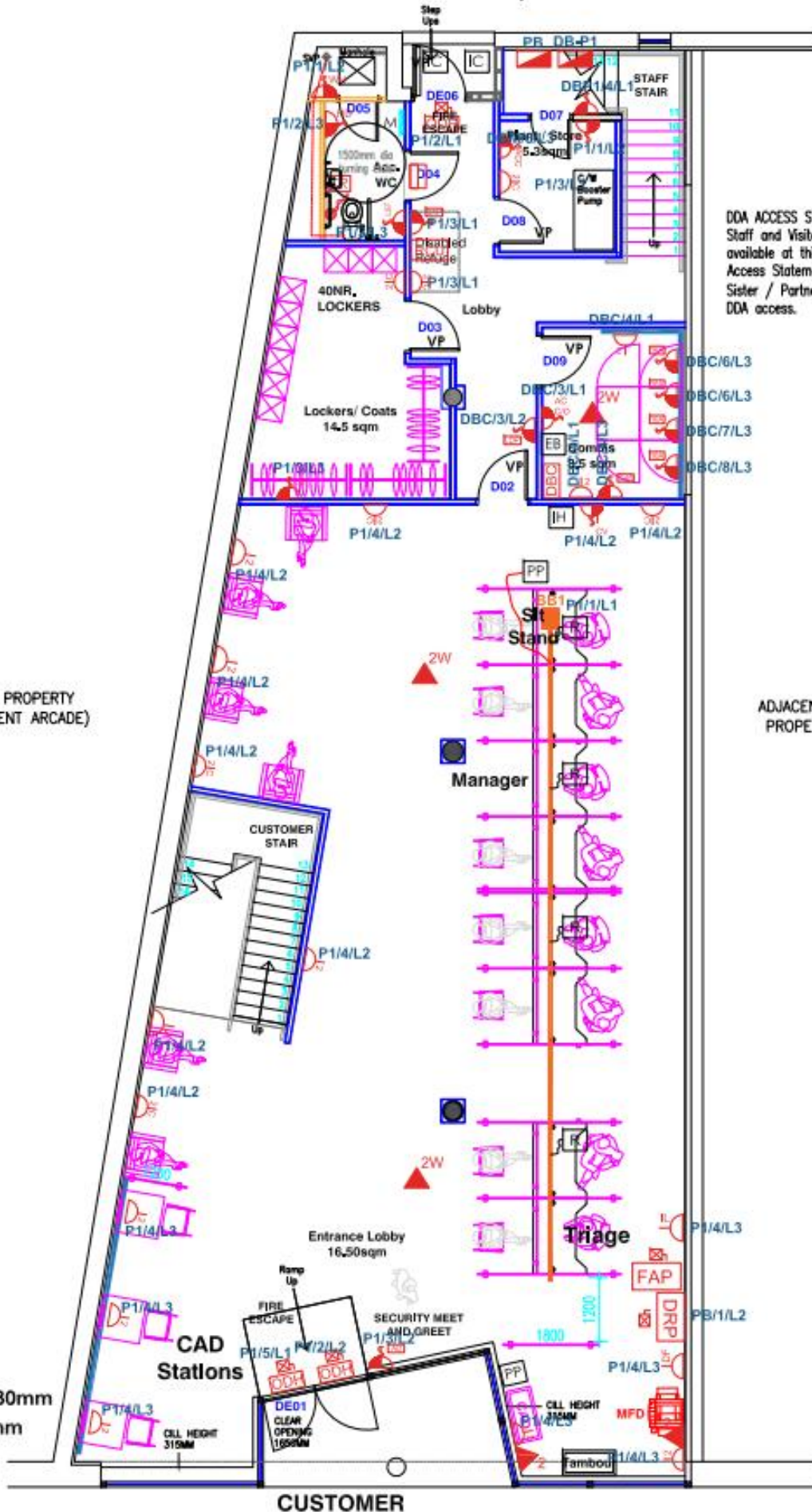
Small Power Layout - Ground Floor
