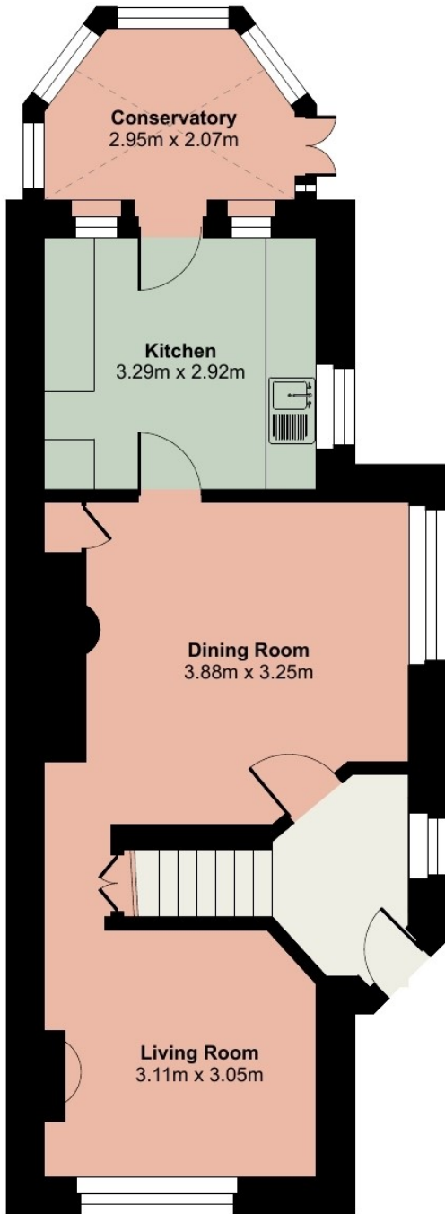
GROUND FLOOR
