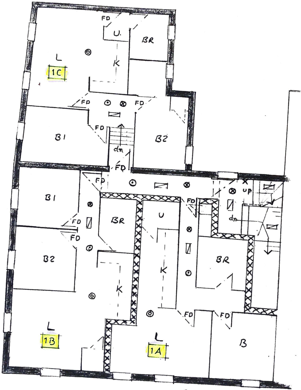
FLATS 1A, B, C FIRST FLOOR PLAN
