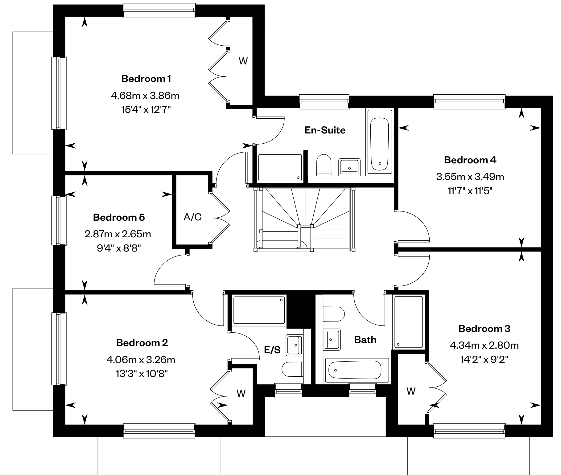
First floor
