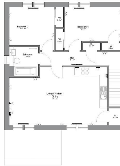
First Floor Apartment
