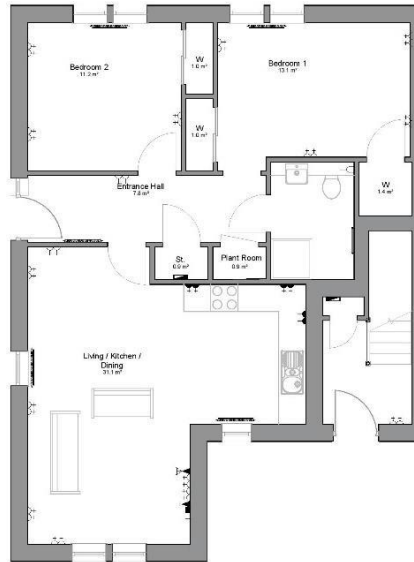
Ground Floor Apartment
