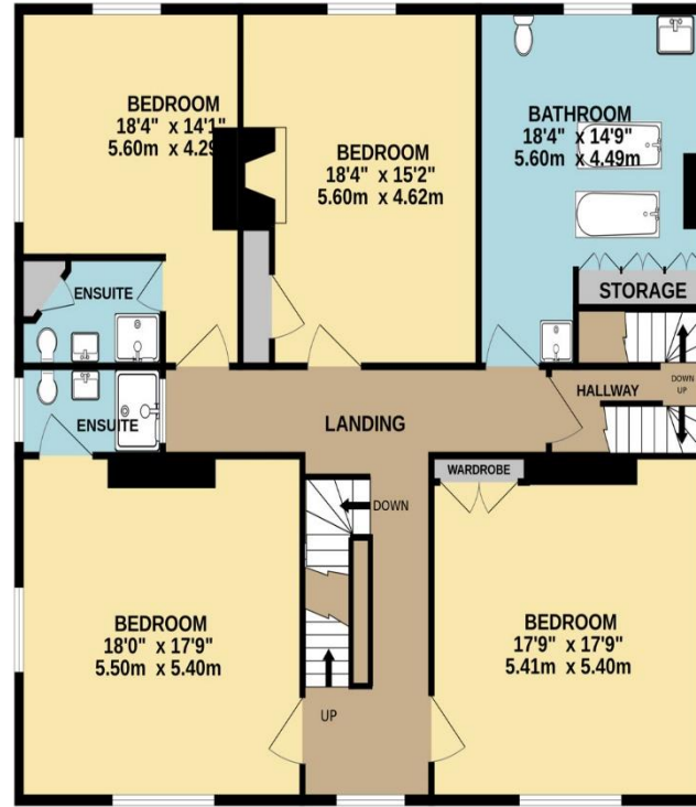
1ST FLOOR 1727 sq.ft. (160.4 sq.m.) approx.
