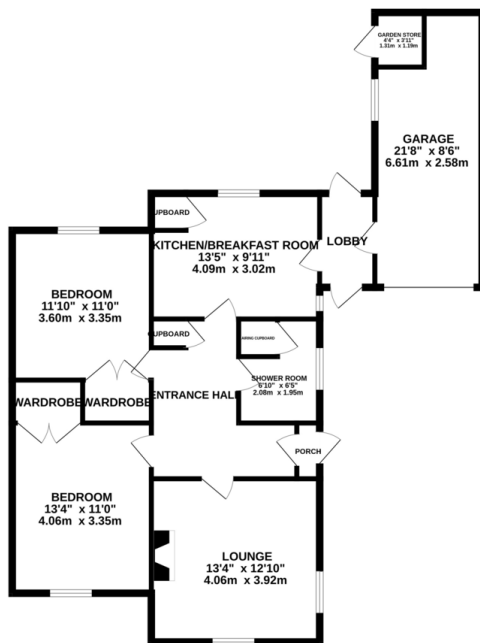
GROUND FLOOR 994 sq.ft. (92.4 sq.m.) approx.
