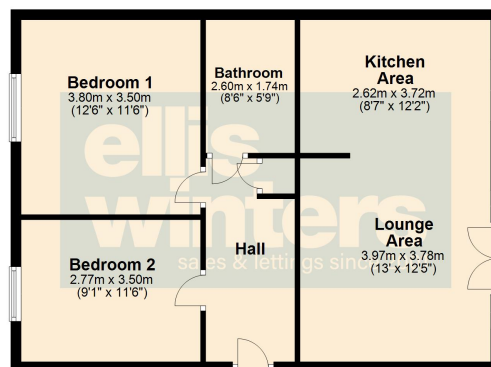
Total area: approx. 61.4 sq. metres (661.0 sq. feet)
