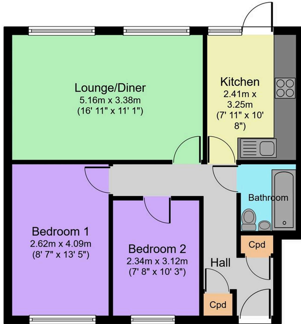
Ground Floor
