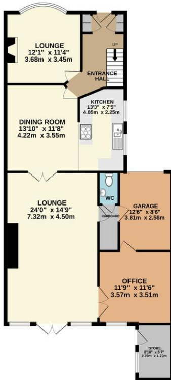
GROUND FLOOR 1152 sq.ft. (107.9 sq.m.) approx.
