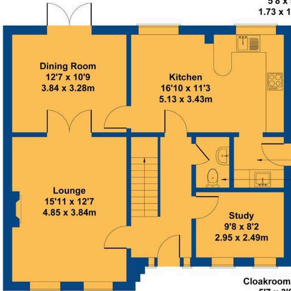
GROUND FLOOR
