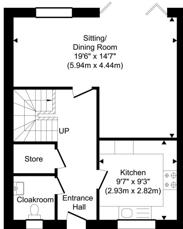
Ground Floor Approximate Floor Area 477.59 sq. ft. (44.37 sq. m)
