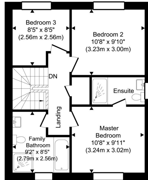
First Floor Approximate Floor Area 477.59 sq. ft. (44.37 sq. m)
