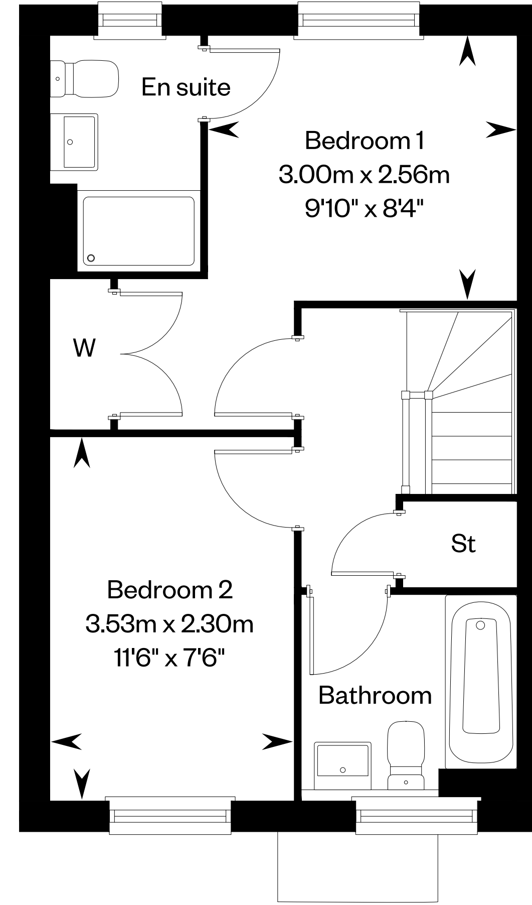
First floor
