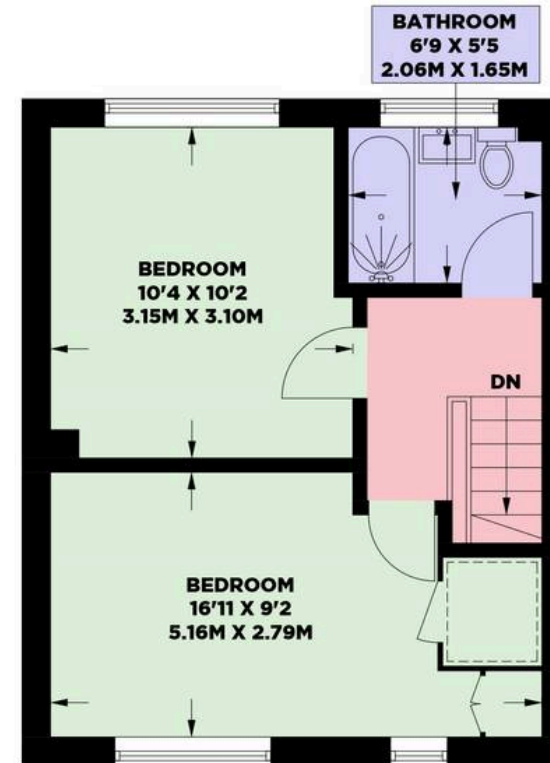
First Floor 360 sq Ft / 33.5 sq M
