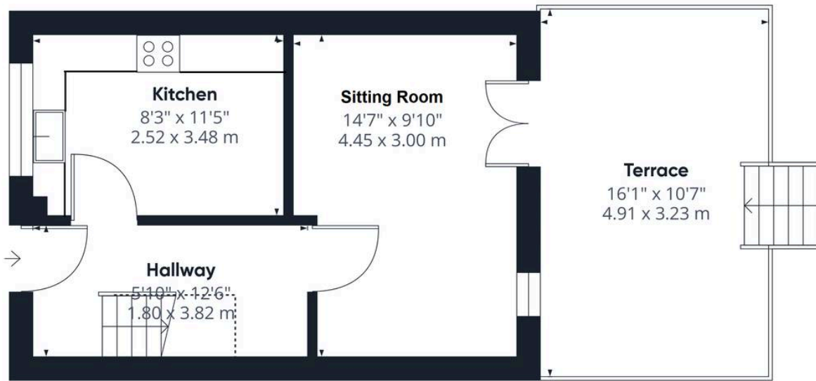
Ground Floor
