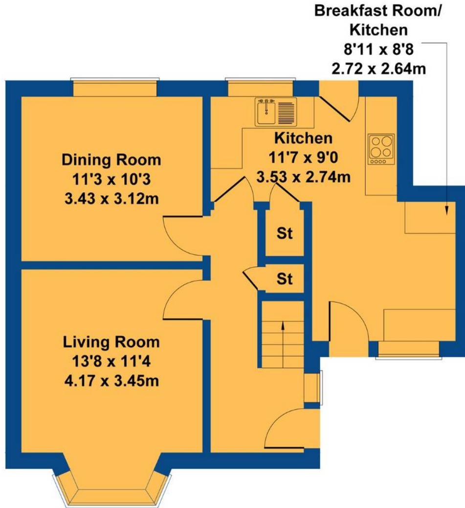
GROUND FLOOR
