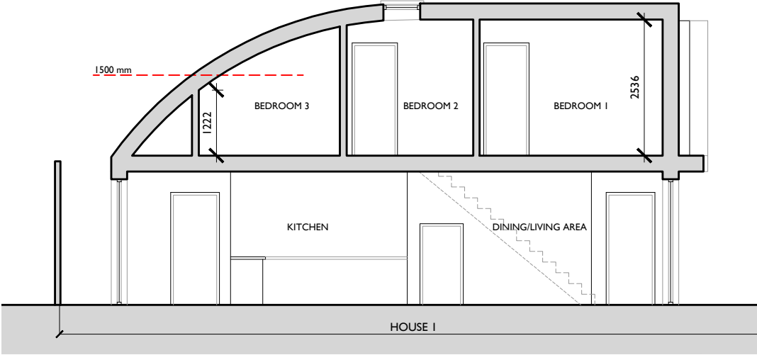
+SX Proposed section AA - scale 1:100 at A3
