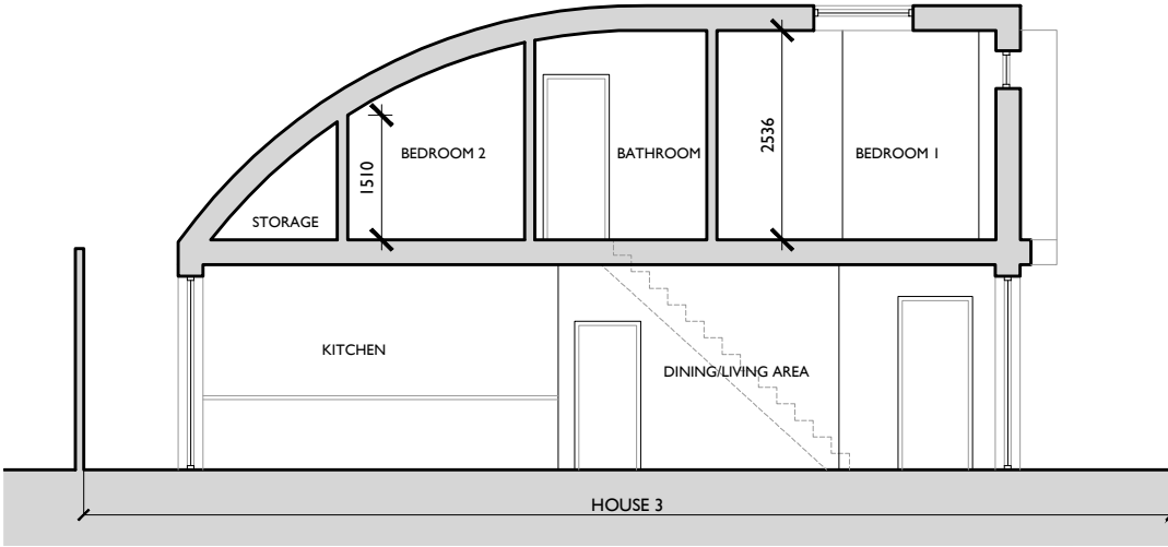
+SX Proposed section BB - scale 1:100 at A3
