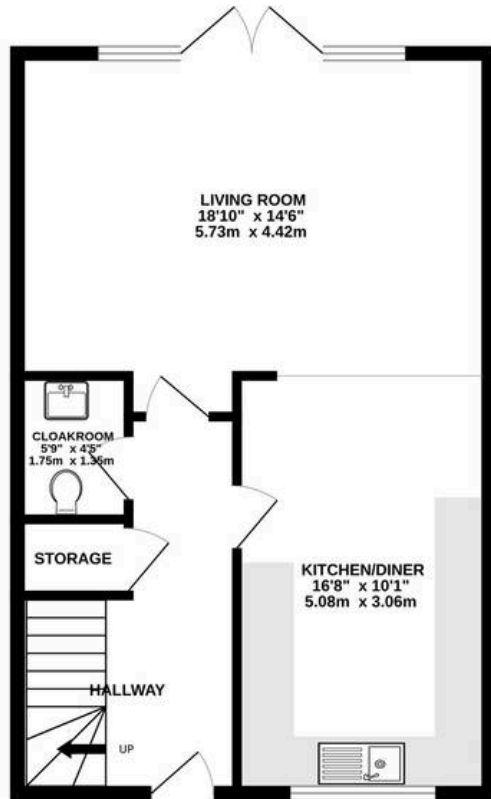
GROUND FLOOR 555 sq.ft. (51.6 sq.m.) approx.
