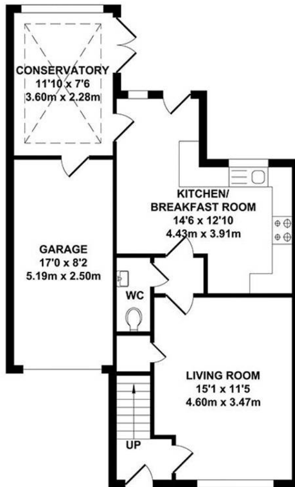
GROUND FLOOR APPROX. FLOOR AREA 660 SQ.FT. (61.36 SQ.M.)
