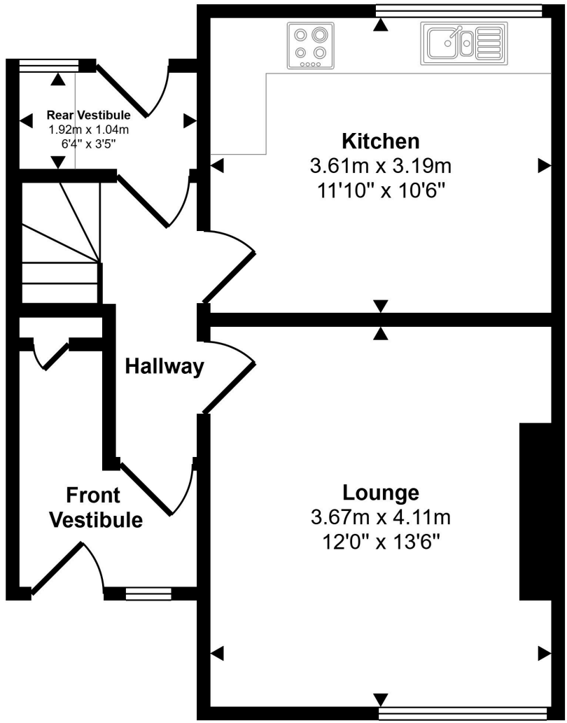
Ground Floor Approx 39 sq m / 416 sq ft
