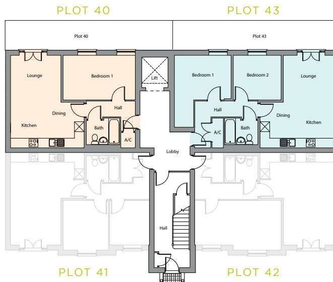
GROUND FLOOR BLOCK 2
