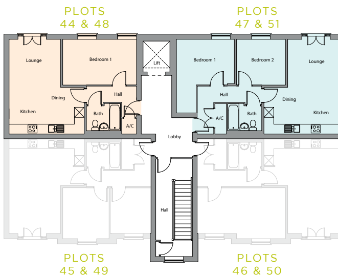
FIRST & SECOND FLOOR BLOCK 2
