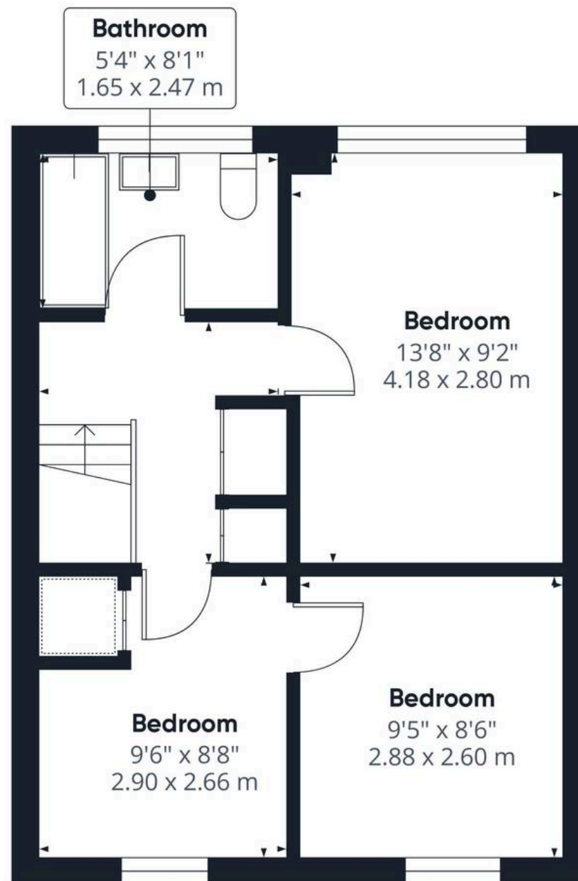
Floor 1 Building 1
