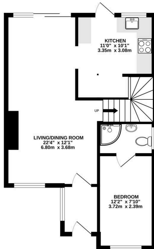
GROUND FLOOR 495 sq.ft. (46.0 sq.m.) approx.
