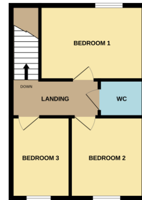
1ST FLOOR 371 sq.ft. (34.5 sq.m.) approx.
