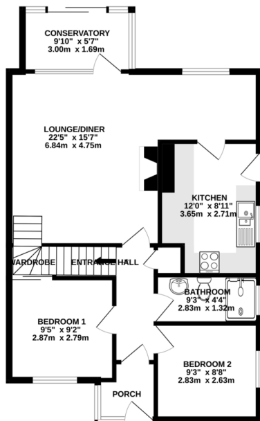
GROUND FLOOR 715 sq.ft. (66.5 sq.m.) approx.
