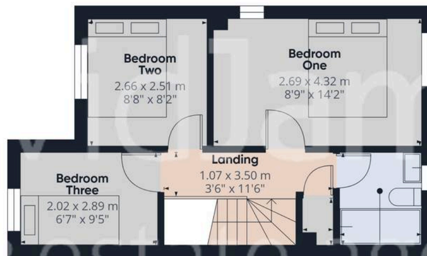
Floor 0
