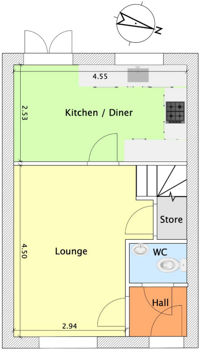
Indicative floor plans for illustration purposes only Approximate Gross Internal Floor Area 676 ft2 / 62.8 m2
