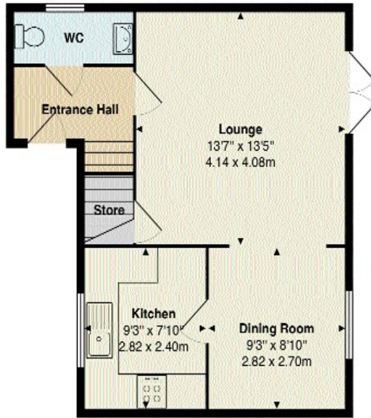
Ground Floor Area: 420 ft 2 ... 39.0 m 2
