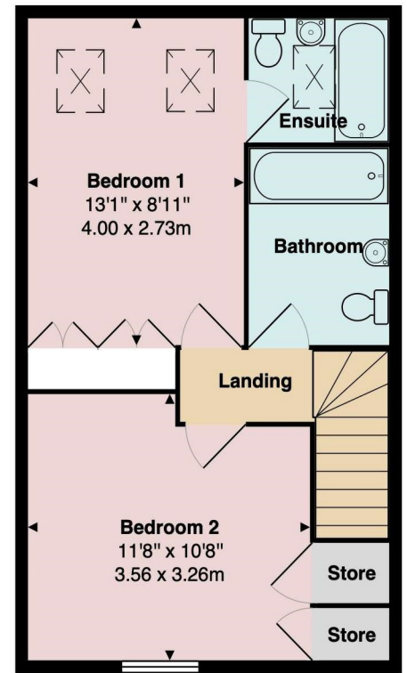
2nd Floor Area: 386 ft 2 ... 35.8 m 2
