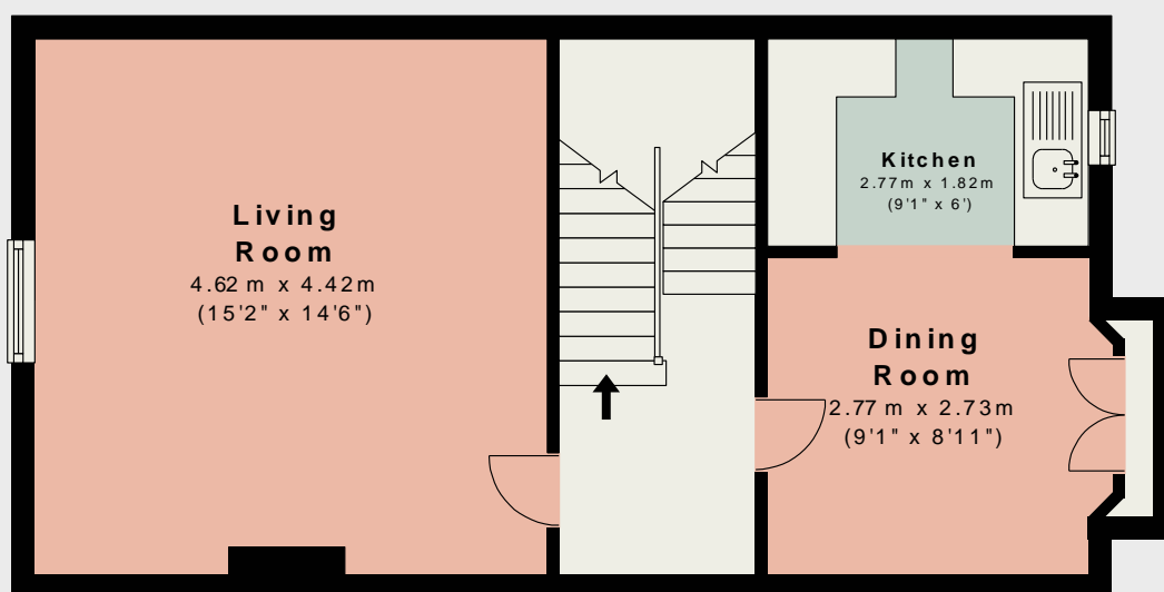
First Floor
