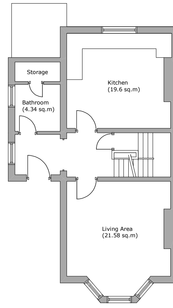
Ground Floor As Existing
