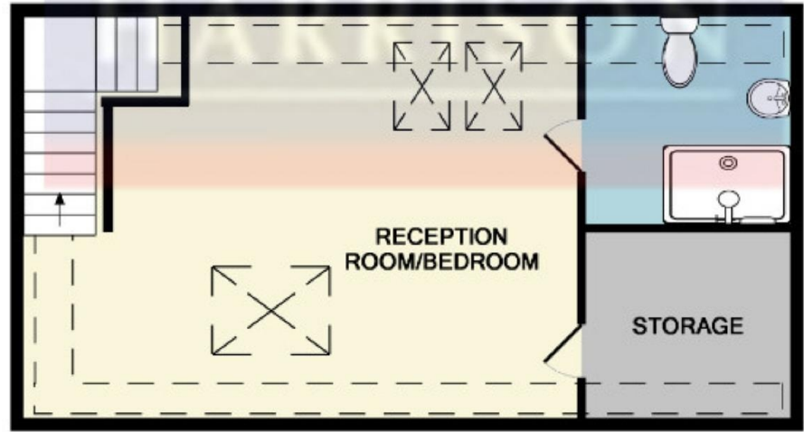
1ST FLOOR
