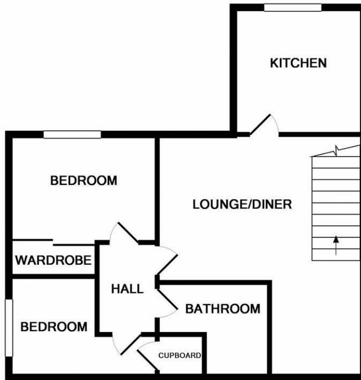
1ST FLOOR
