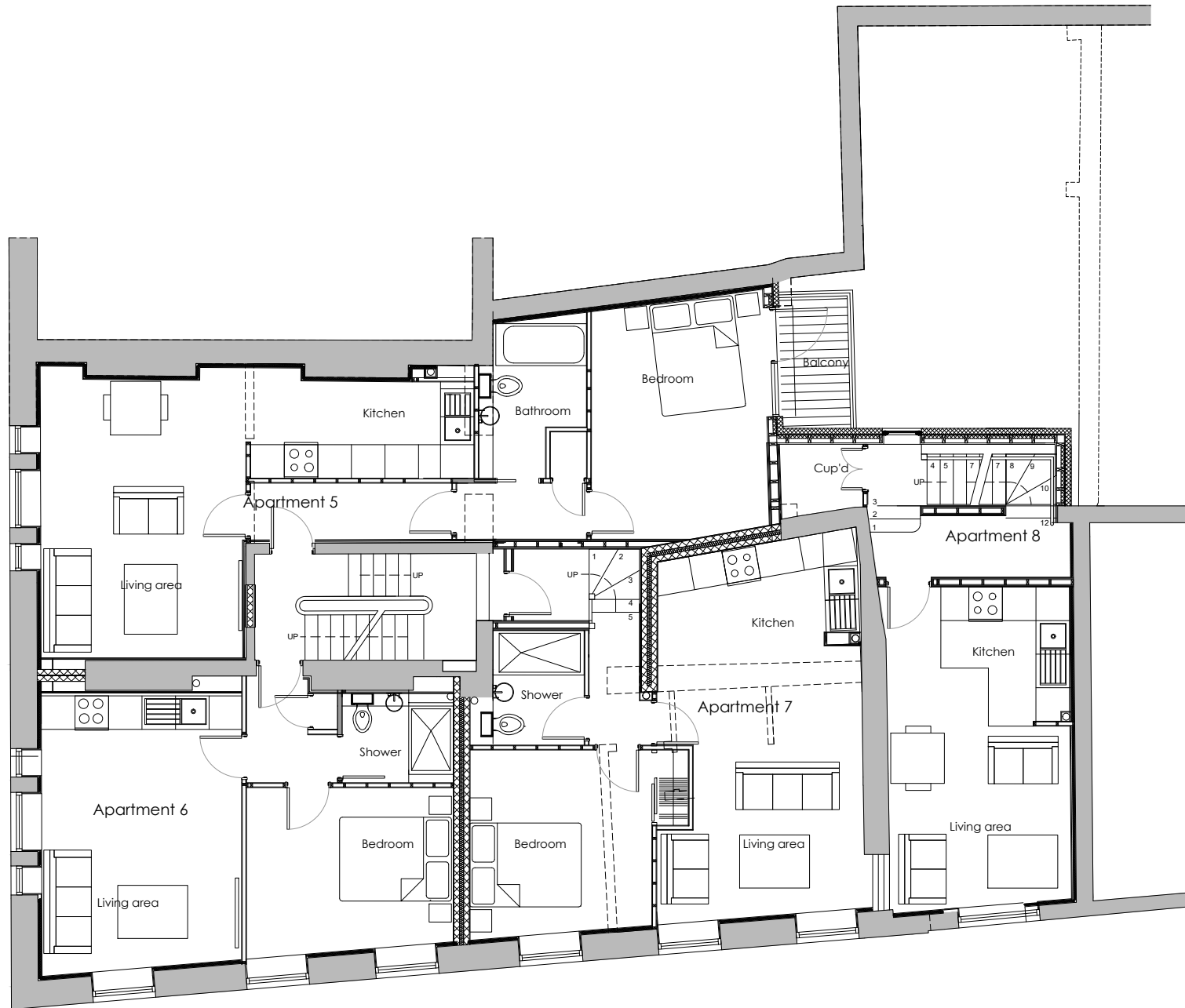
FIRST FLOOR
