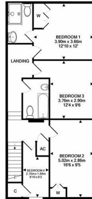
FIRST FLOOR APPROX. FLOOR AREA 69.1 SQ.M. (744 SQ.FT.)
