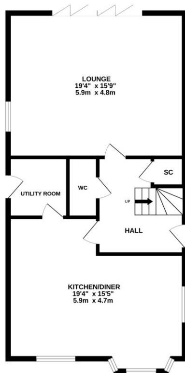
GROUND FLOOR 740 sq.ft. (68.8 sq.m.) approx.
