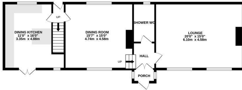
GROUND FLOOR 820 sq.ft. (76.2 sq.m.) approx.
