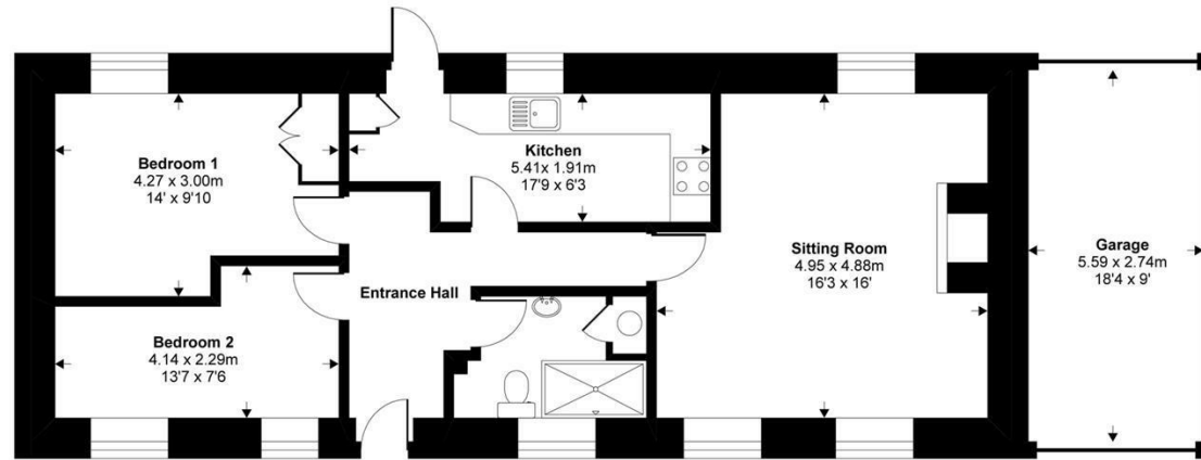
Ground Floor
